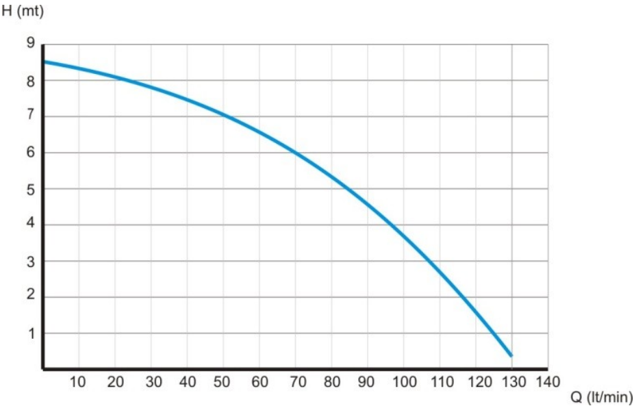
Fig. 6 LIFTING EFFECTIVENESS
