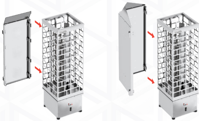
Wall Installation with Protective Cover
