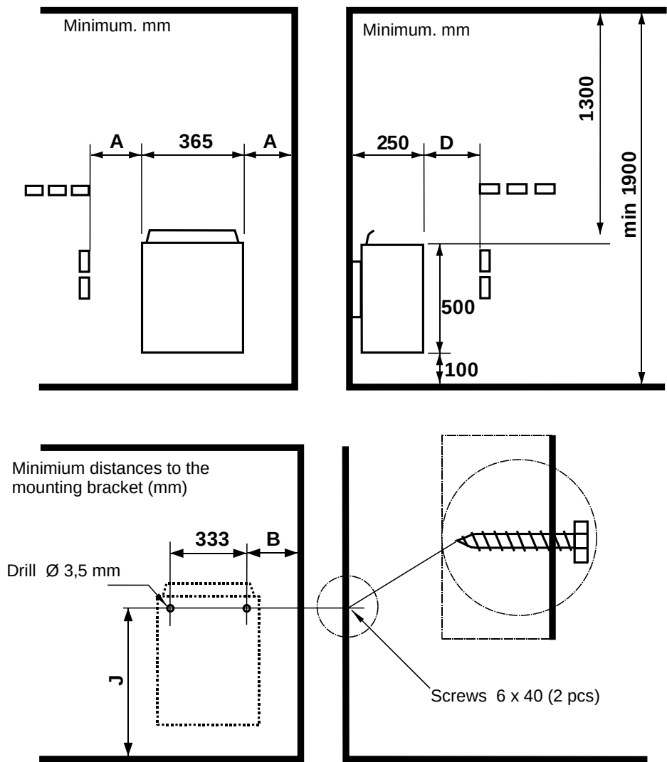
Image 2 Safety distances, dimensions minimum dimensions (mm)
