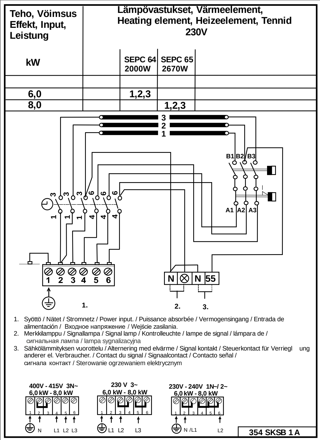
Image 4 Viring diagram
